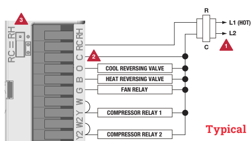
Typical 2H/2C Heat Pump System w/o Aux.
