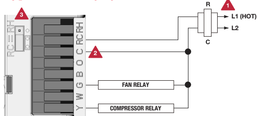
Typical Cool-Only System
