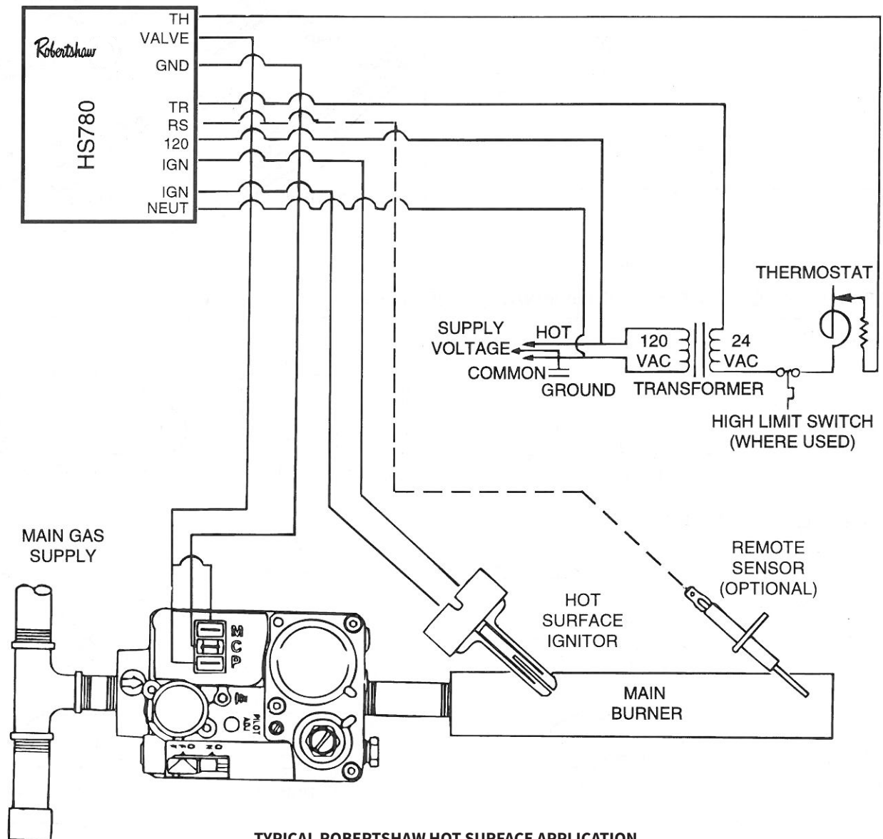
TYPICAL ROBERTSHAW HOT SURFACE APPLICATION
