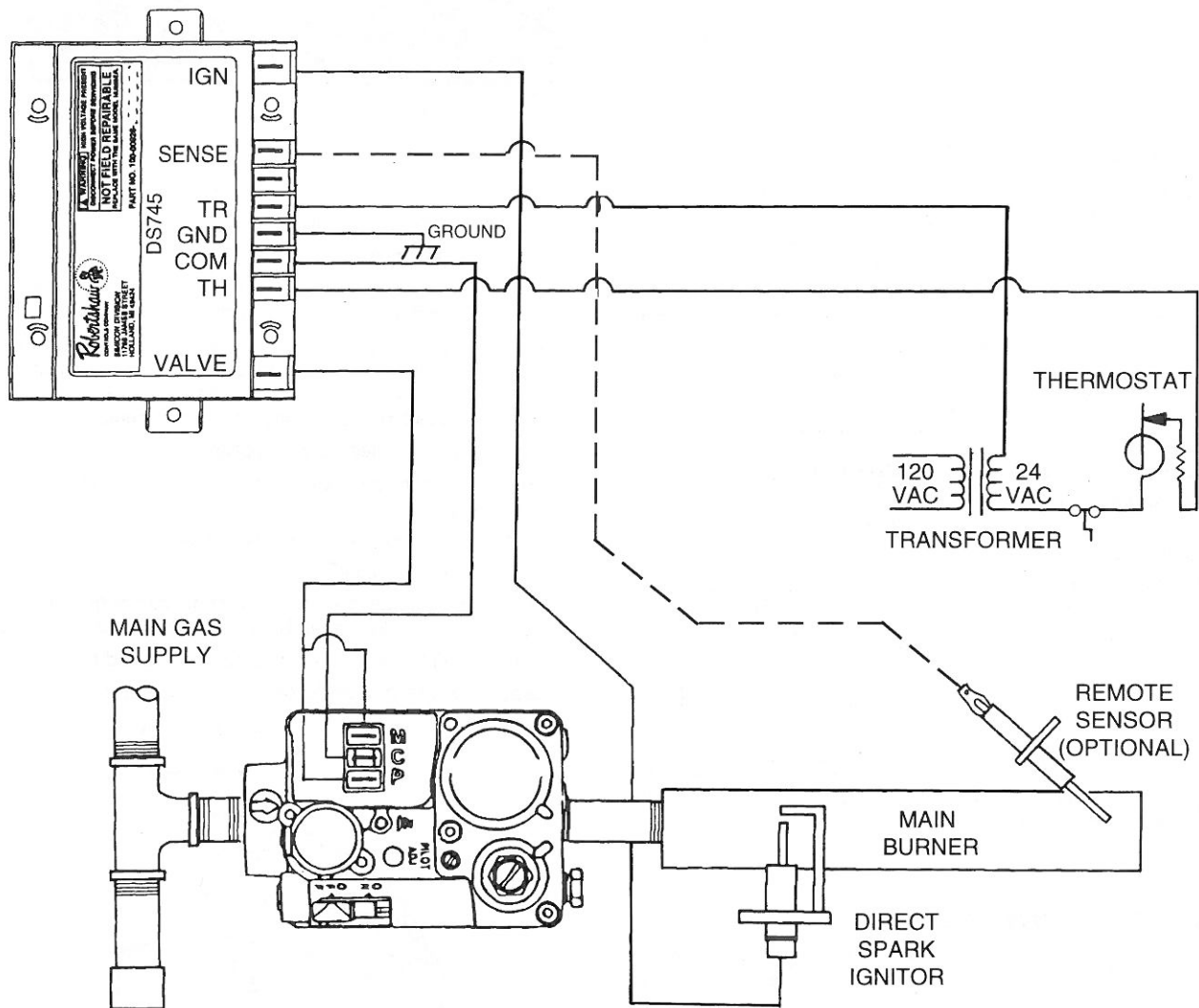
TYPICAL ROBERTSHAW DIRECT SPARK APPLICATION
