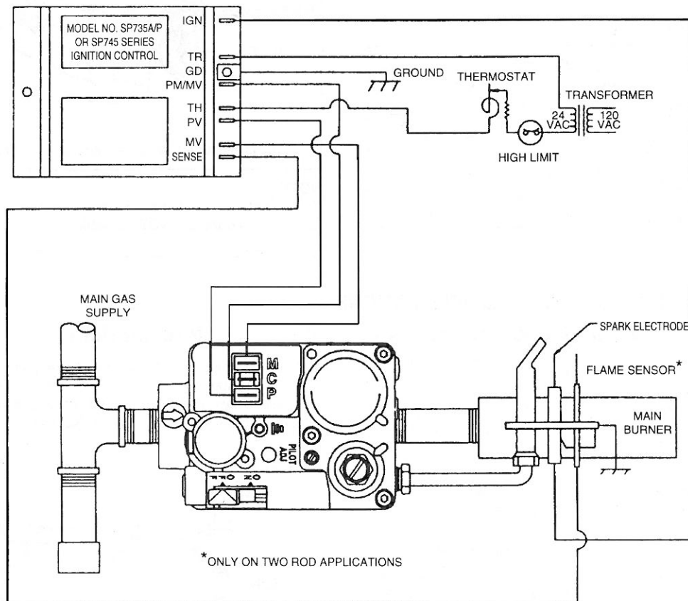
TYPICAL ROBERTSHAW INTERMITTENT PILOT APPLICATION
